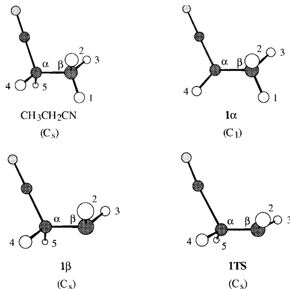
Figure 1. Calculated MP2/6-31+G(d) structures for CH 3 CH 2 CN, 1 \alpha , 1 \beta , and ITS .
